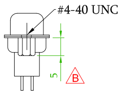
Rear rivet #4-40, H=5.0
