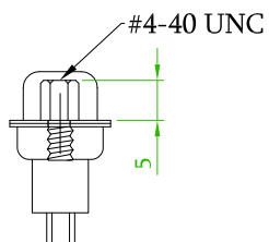
Thread Insert #4-40+ Jack Screw #4-40 Removable
