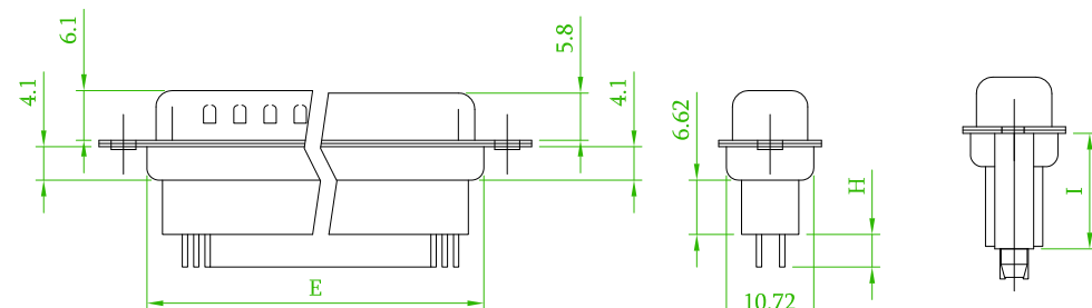
W/O Boardlock
