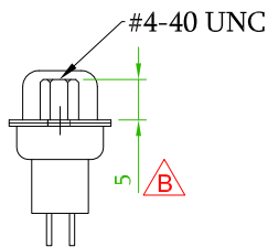
Front rivet #4-40, H=5.0
