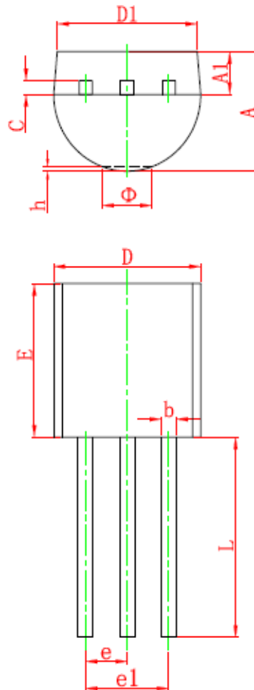
TO-92 PACKAGE OUTLINE DIMENSIONS
