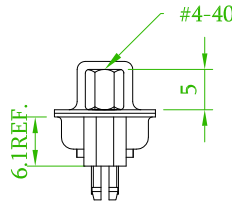
With Boardlock +Thread Insert #4-40 +Jack Screw #4-40 Removable 57DBDSXM-XXCCXXXXA-XX
