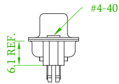
With Boardlock +Thread Insert #4-40 57DBDSXM-XXBAXXXA-XX
