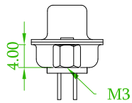
Rear Rivet M3, H:4.0 57DBDSXM-XXNGXXXXA-XX
