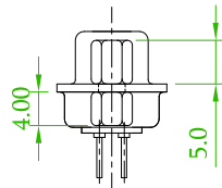
Rear Rivet 4.0mm + Jack Screw #4-40 Removable 57DBDSXM-XXNLXXXXA-XX
