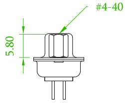
Front Rivet #4-40, H:5.8 57DBDSXM-XXNHXXXXA-XX
