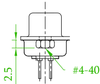
Rear Rivet #4-40, H:2.5 57DBDSXM-XXN1XXXXA-XX
