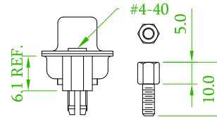
With Boardlock +Thread Insert #4-40 +Jack Screw #4-40 Removable 57DBDSXM-XXCCXXXXA-XX
