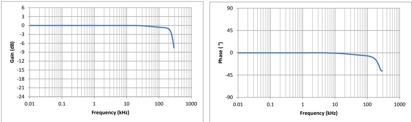
Figure 5: Typical frequency response, small signal bandwidth
