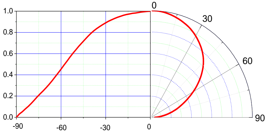
Fig 2. Viewing Angle Distribution, I_F = 20\text{mA}
