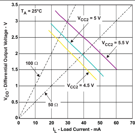
Figure 11. Driver Differential Output Voltage vs Load Current
