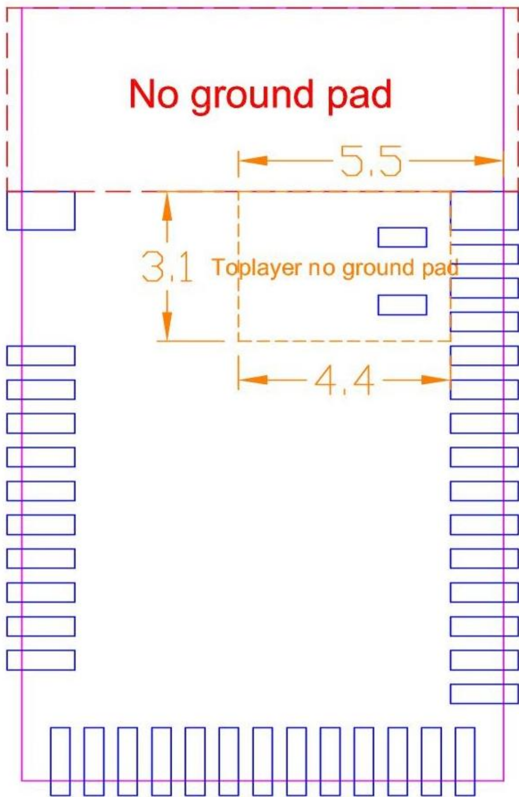
Toplayer no ground pad
