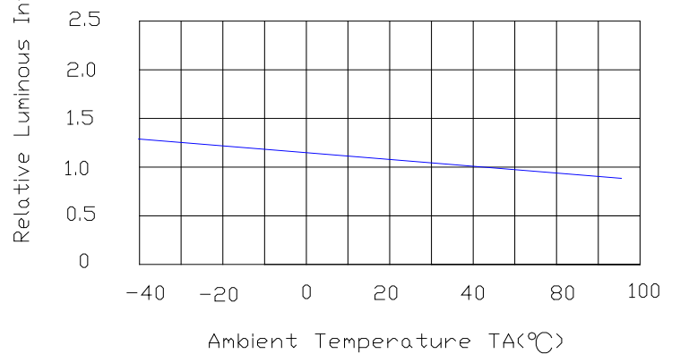
Luminous Intensity Vs. Ambient Temperature
