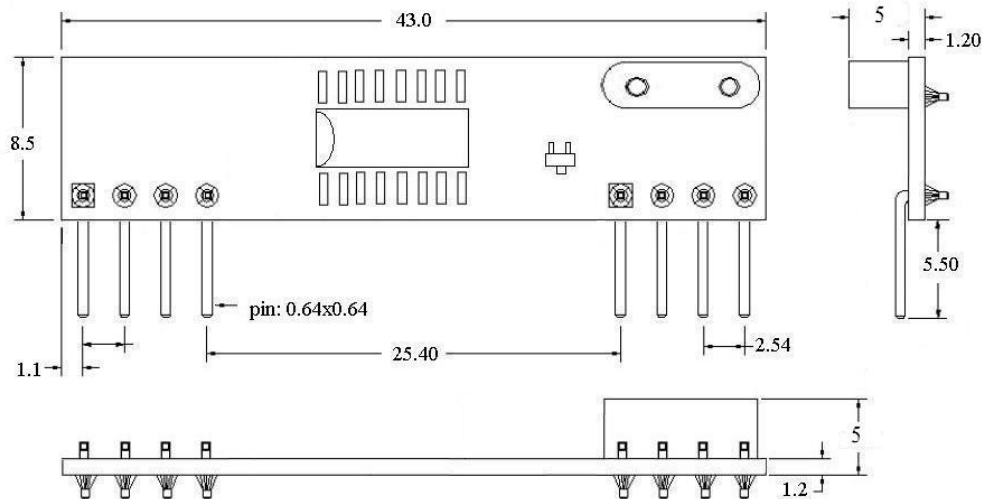
Figure2 CY02 Dimension
