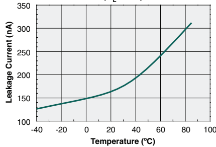
Leakage Current vs. Temperature ( V_L=60\text{V} )
