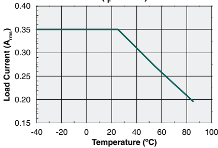
Maximum Load Current vs. Temperature ( I_F=10mA )
