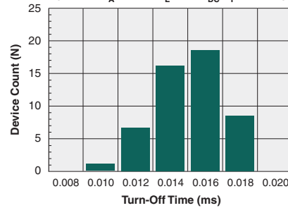
Typical Turn-Off Time (N=50, T_A=25^\circ C , I_L=0.5A_{DC} , I_F=10mA )
