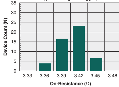
Typical On-Resistance Distribution (N=50, T_A=25^\circ C , I_L=0.5A_{DC} , I_F=10mA )
