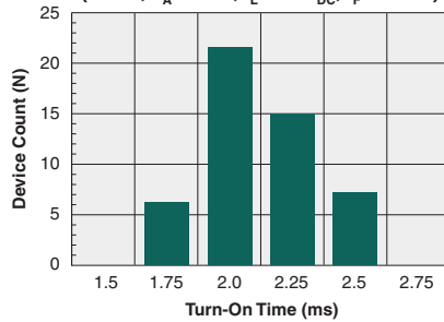
Typical Turn-On Time (N=50, T_A=25^\circ C , I_L=0.5A_{DC} , I_F=10mA )
