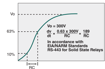
dV/dt Method
