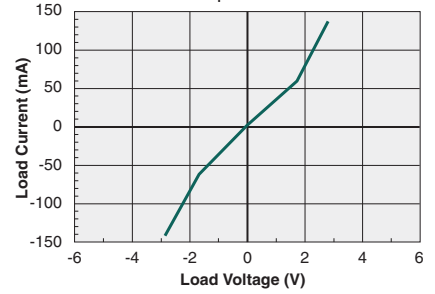
Typical Load Current vs. Load Voltage (I F =0mA)
