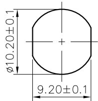
Panel cut
