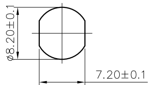
Panel cut
