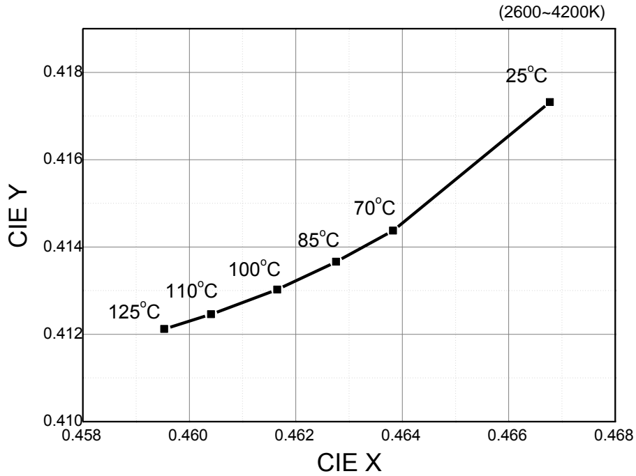
Fig 8. Chromaticity Coordinate vs. Junction Temperature, I_F=150mA
