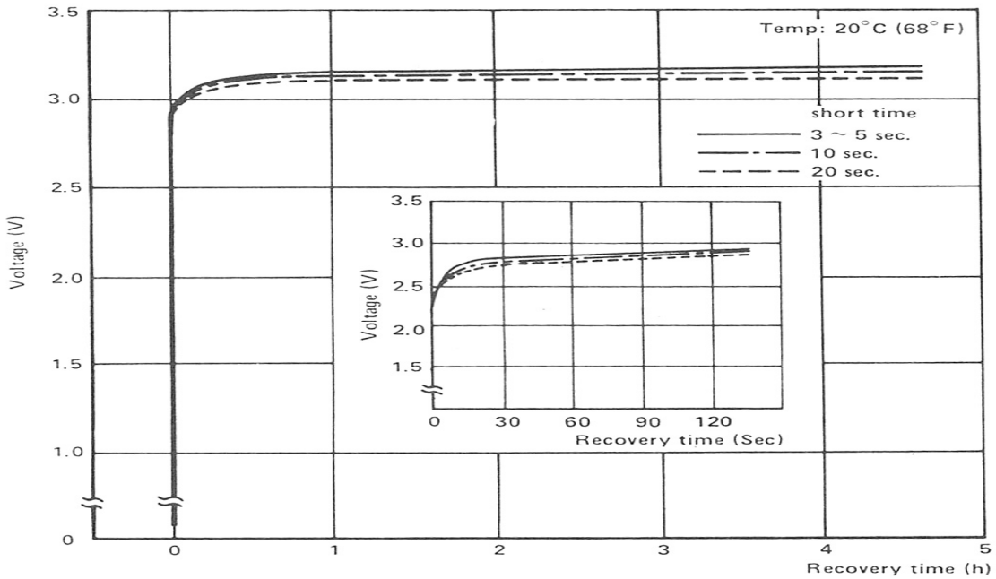
Fig. 1 Voltage recovery characteristics after short test
