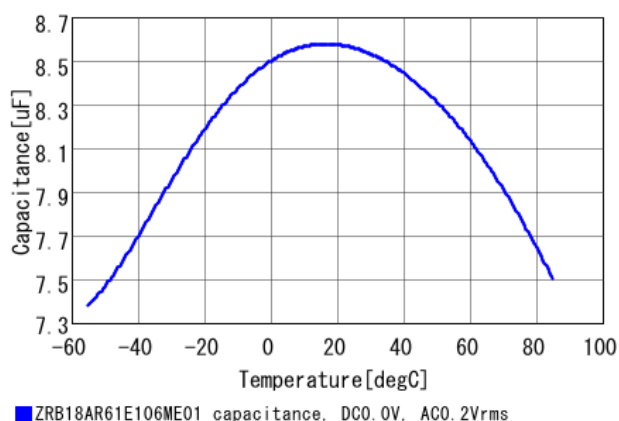
Tempeture Characteristics
