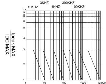
tp-PULSE DURATION \mu S (5)
