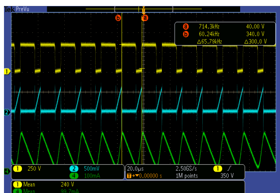
Crucial waveforms
