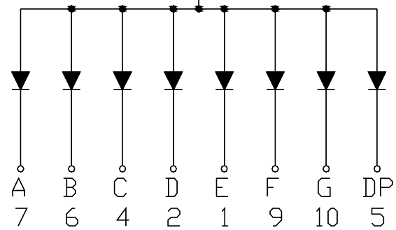
Common Anode
