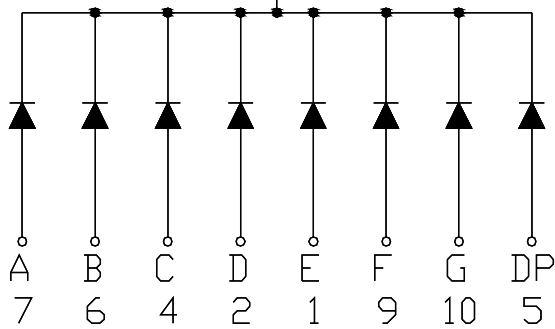
Common Cathode
