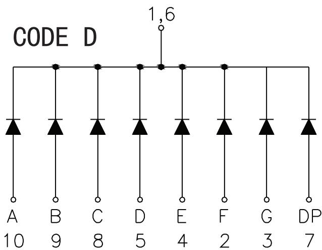
COMMON CATHODE
