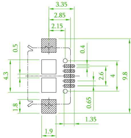
Recommended PCB Layout (PCB TOLERANCE ±0.1)
