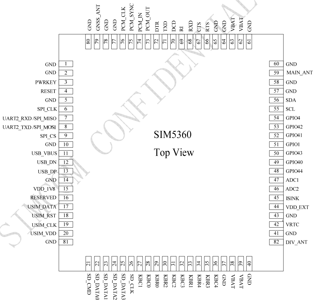
Figure 2: Pin view
