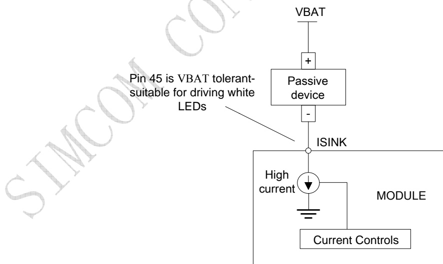
Figure 37: Current drive
