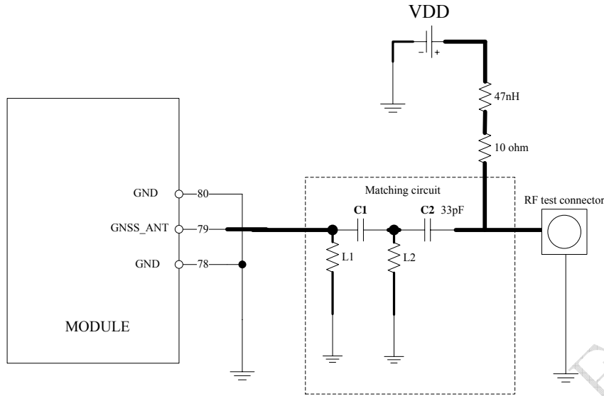
Figure 35: Active antenna circuit
