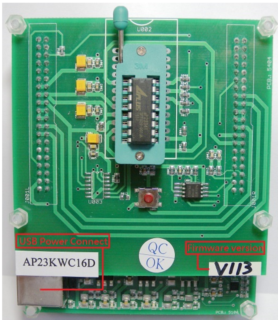
Fig. 1 The aP23KWC16D USB Writer Programmer Board
