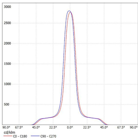
SL-050K-S K:5.71cd/lm,LED:02x
