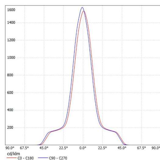
SL-050K-M K:3.23cd/lm,LED:02x
