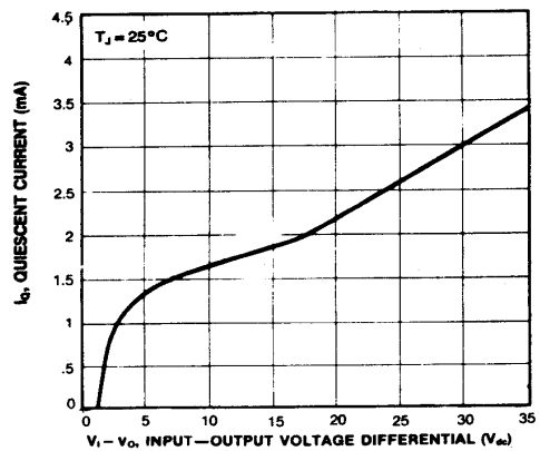
Figure 7. Minimum Load Current
