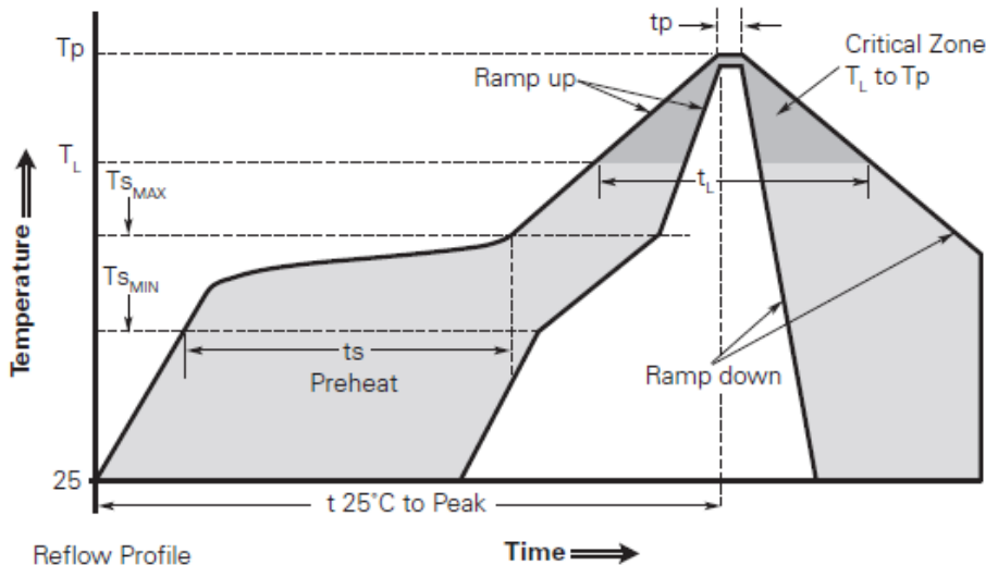
Reflow Profile
