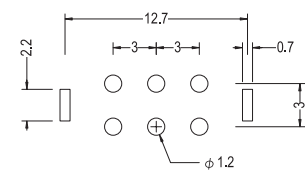
P.C.B. HOLE DETAIL
