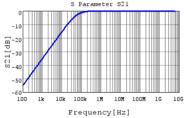
GRM155R71E273KA88 S21 DC0V, 25degC
