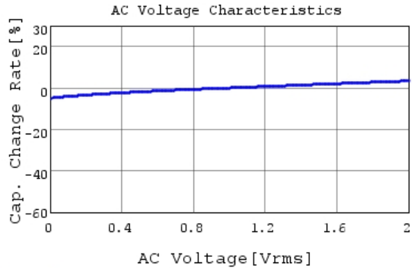
GRM155R71E273KA88 C-AC Voltage capchange, DC
