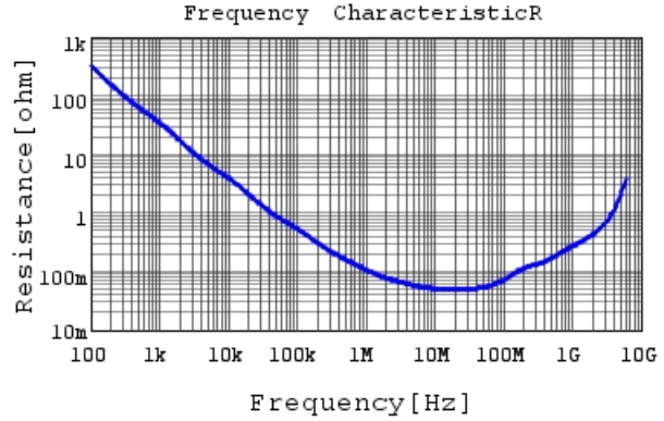
GRM155R71E273KA88 R DC0V, 25degC
