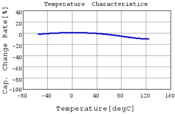
GRM155R71E273KA88 C-Temp. capchange, DC0.0V,
