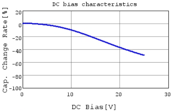
GRM155R71E273KA88 C-DC bias capchange, 25.0c
