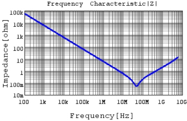
GRM155R71E273KA88 |Z| DC0V, 25degC
