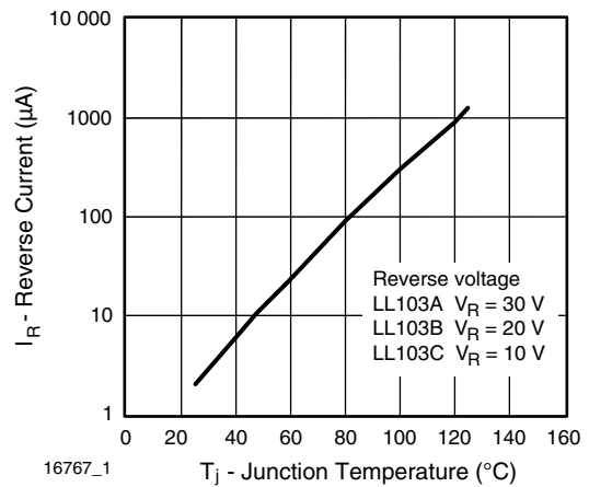
16767_1 Fig. 3 - Reverse Current vs. Junction Temperature
