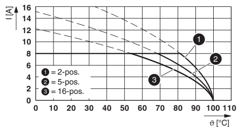
Type: FK-MCP 1,5/...-STF-3,81 with MCD 1,5/...-GF-3,81
