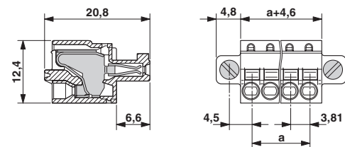
Dimensional drawing
