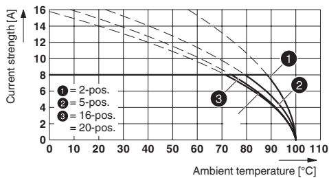
Type: FK-MCP 1,5/...-STF-3,81 with MCV 1,5/...-GF-3,81 P...THR
