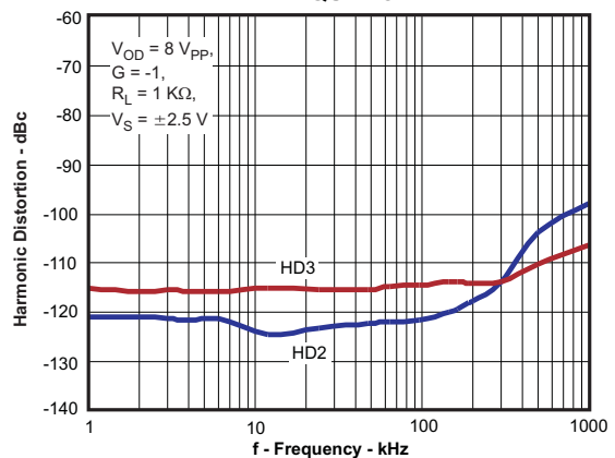
Measured HD 2 /HD 3 for G = -1, V OD = 8 V PP , R L = 1 K \Omega (circuit shown on the left)
