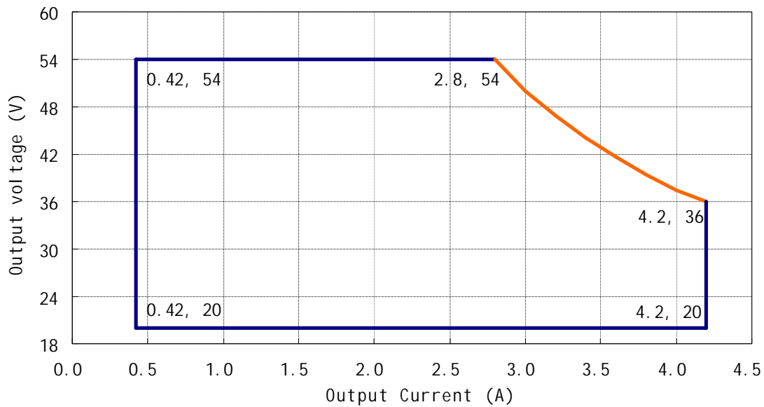
Output Voltage VS Output Current Curve
