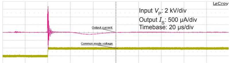
Figure 12: Detail of typical common mode perturbation (2000 V step with 6 kV/μs, R_M = 100 \Omega )
