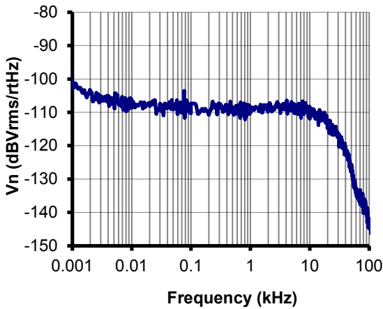
Figure 13: Typical noise voltage density e_{no} with R_M = 50 \Omega
