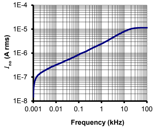
Figure 14: Typical total output rms noise current with R_M = 50 \Omega (fc is upper cut-off frequency of bandpass, low cut off frequency is 1 Hz)
