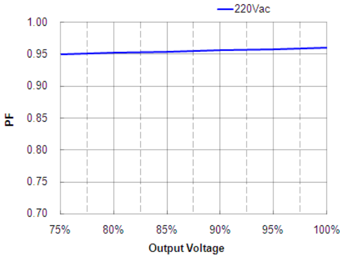
Power Factor vs. Output Voltage
