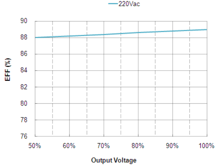
Efficiency vs. Output Voltage
