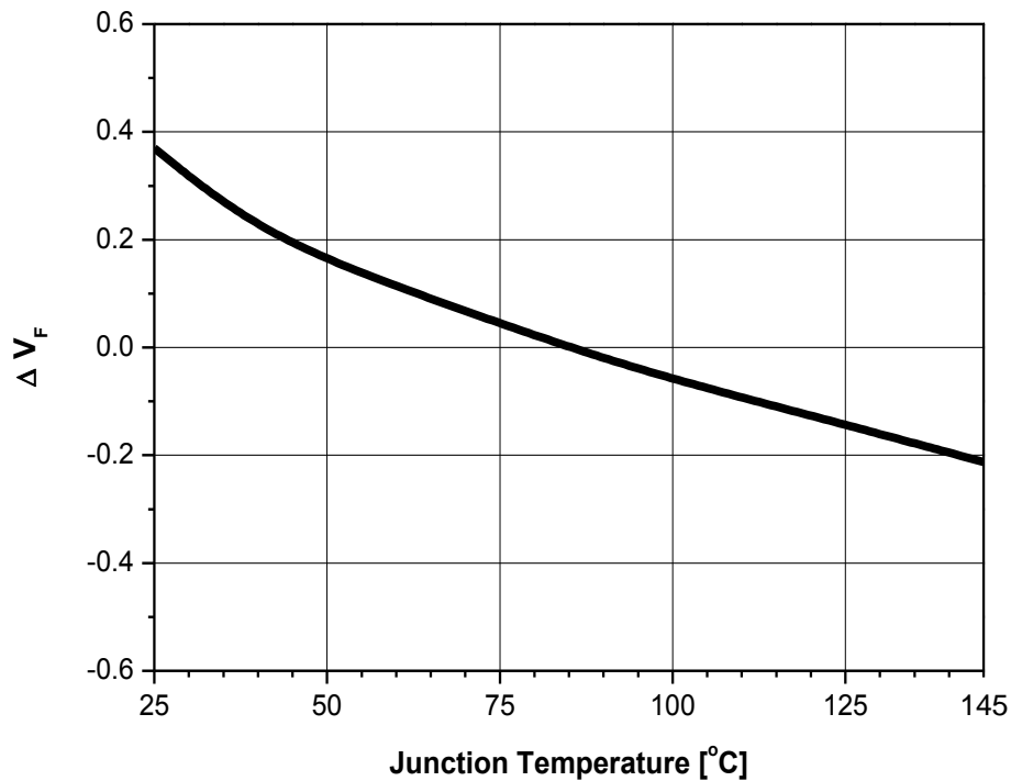
Fig 8b. Relative Forward Voltage vs. Junction Temperature for Y11-XX-XX-C, I_F=115\text{mA}
