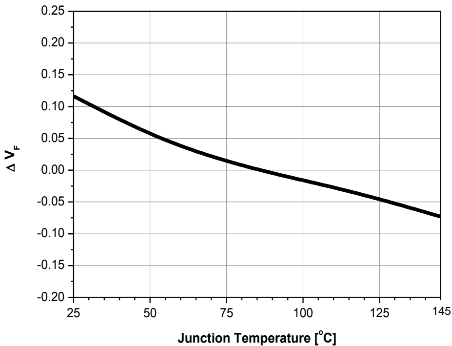
Fig 7. Relative Forward Voltage vs. Junction Temperature, I_F=700\text{mA}
