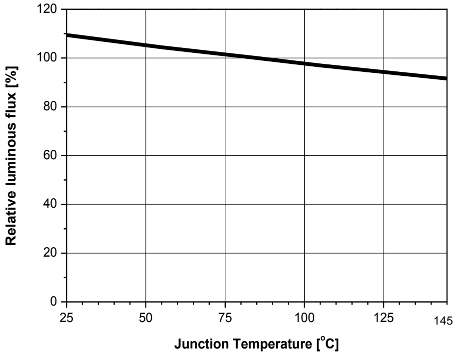
Fig 6. Relative Light Output vs. Junction Temperature, I_F=700\text{mA}
