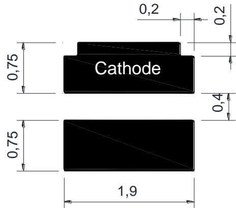
< Recommended Solder Pattern >
