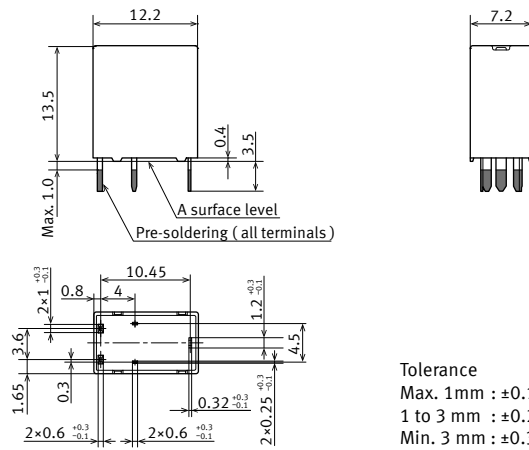
External dimensions
