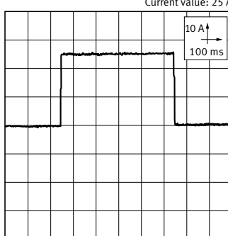
Load current waveform Current value: 25 A
