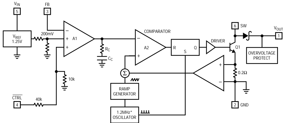
Figure 2. YT2665 Block Diagram
