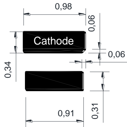
< Recommended Solder Pattern >
