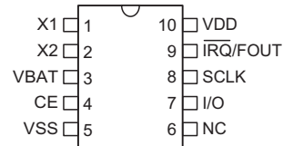
HT1382 10 MSOP-A
