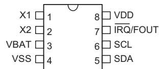
HT1382 8 DIP-A/SOP-A/MSOP-A
