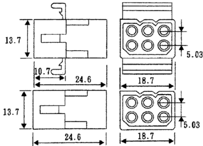
5H5030F0-203WBL00D01 2x3 Pin, W/O Ear
