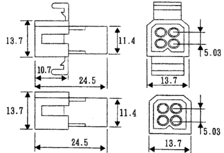
5H5030F0-202WBL00D01 2x2 Pin, W/O Ear
