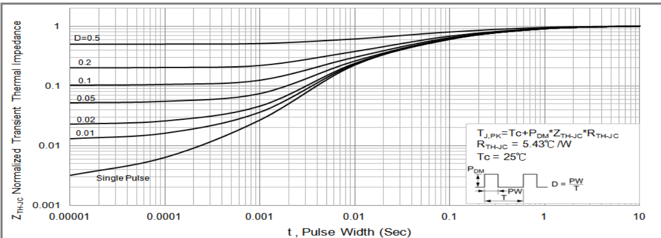
Fig.15 PJF4NA60H Normalized Transient Thermal Impedance vs. Pulse Width
