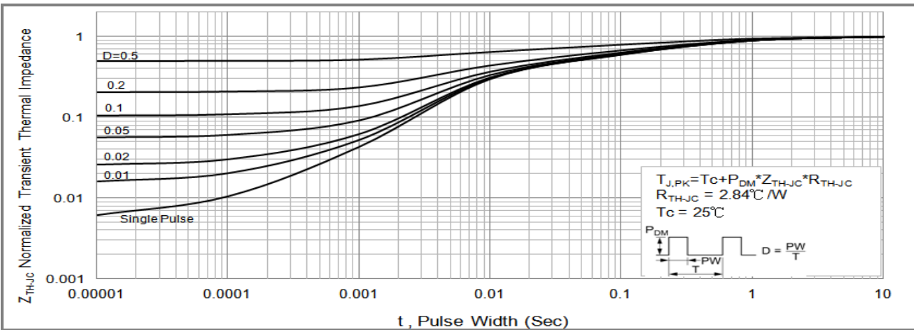
Fig.14 PJP4NA60H Normalized Transient Thermal Impedance vs. Pulse Width
