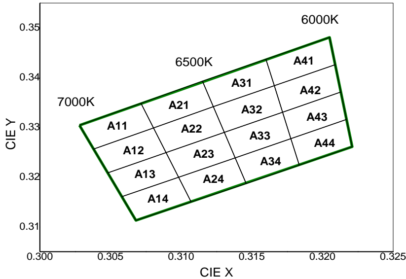
CIE Chromaticity Diagram (Cool white), T_j=25^\circ\text{C} , I_F=200\text{mA}
