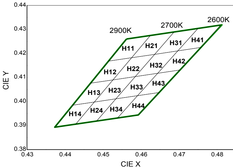
CIE Chromaticity Diagram (Warm white), T_j=25^\circ\text{C} , I_F=200\text{mA}
