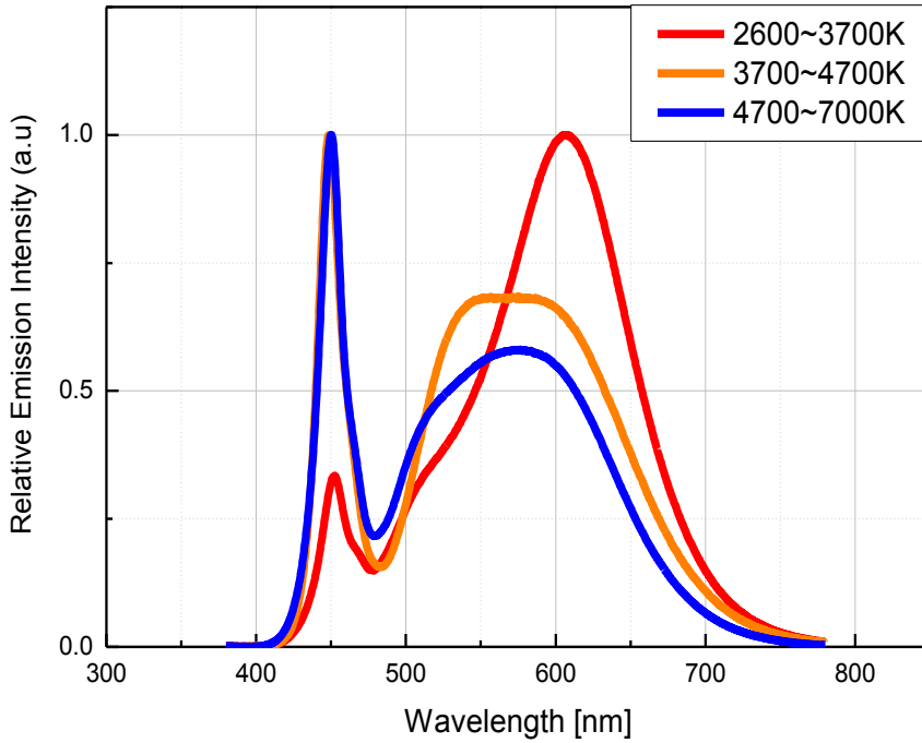
Fig 1. Color Spectrum, T_j = 25^\circ\text{C} , I_F = 200\text{mA}
