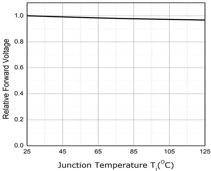
Fig 7. Junction Temperature vs. Relative Forward Voltage, I_F=200\text{mA}
