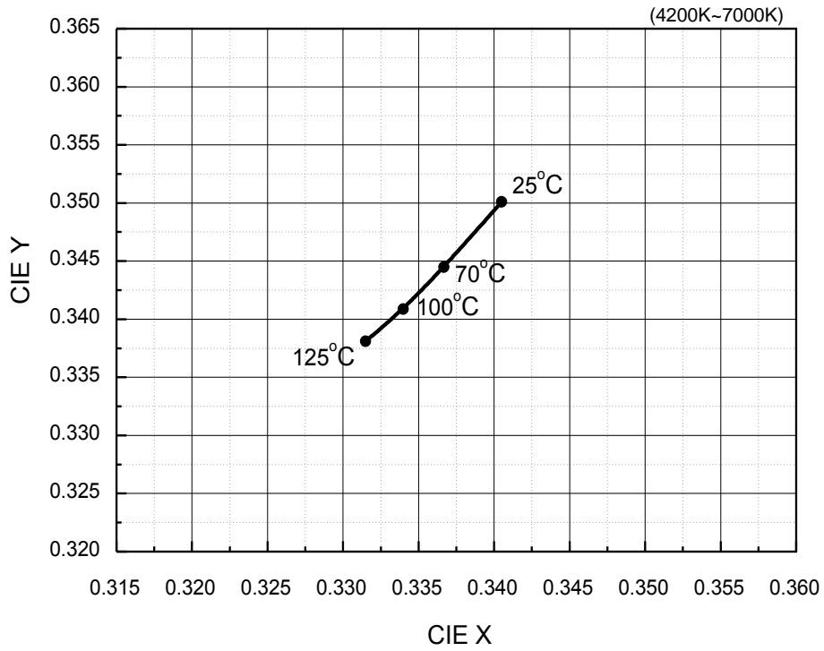
Fig 8. Chromaticity Coordinate vs. Junction Temperature, I_F=200\text{mA}
