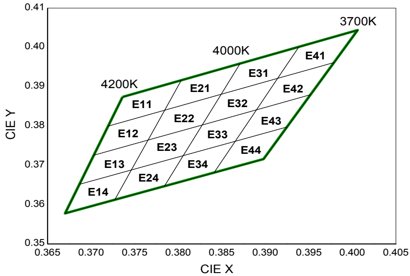
CIE Chromaticity Diagram (Neutral white), T_j=25^\circ\text{C} , I_f=200\text{mA}
