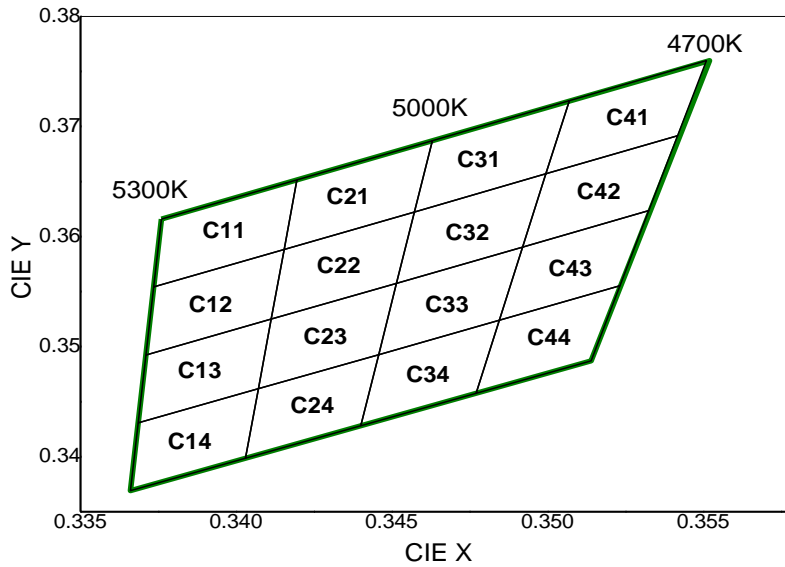
CIE Chromaticity Diagram (Cool white), T_j=25^\circ\text{C} , I_f=200\text{mA}
