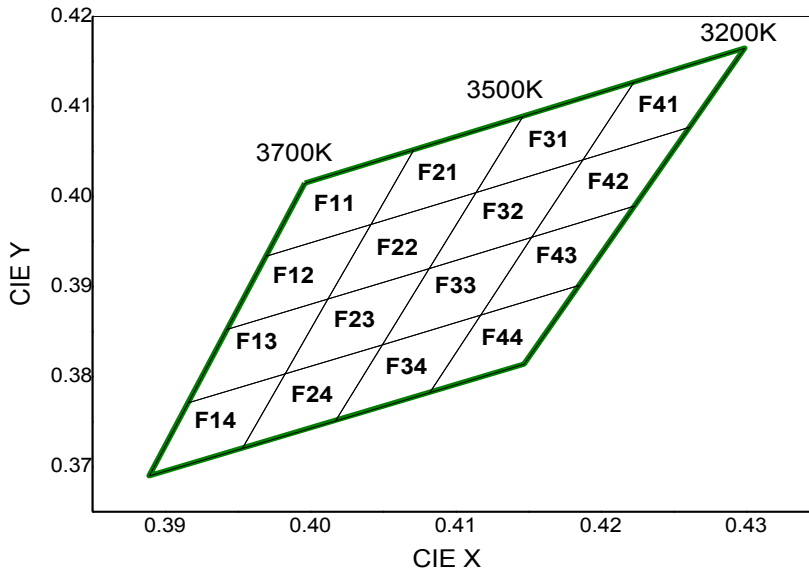
CIE Chromaticity Diagram (Warm white), T_j=25^\circ\text{C} , I_F=200\text{mA}
