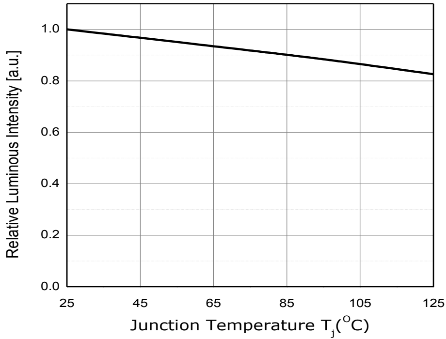
Fig 6. Junction Temperature vs. Relative Luminous Intensity, I_F=200\text{mA}
