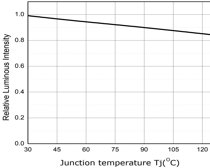
Fig 6. Junction Temperature vs. Relative Luminous Intensity, I_F=32\text{mA}
