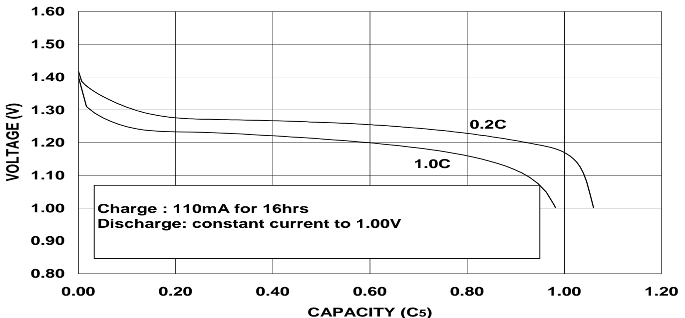
DISCHARGE CHARACTERISTICS OF BPI-48AA1100mAh CELL
