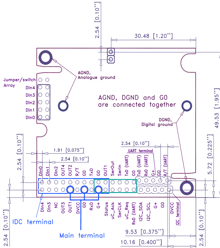
Figure 1. CO 2 Engine® K30 FR I/O notations, terminal positions and some important dimensions for mounting the K30 platform PCB into a host system (Top view).
