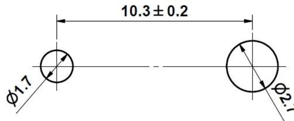
MOUNTING HOLES
