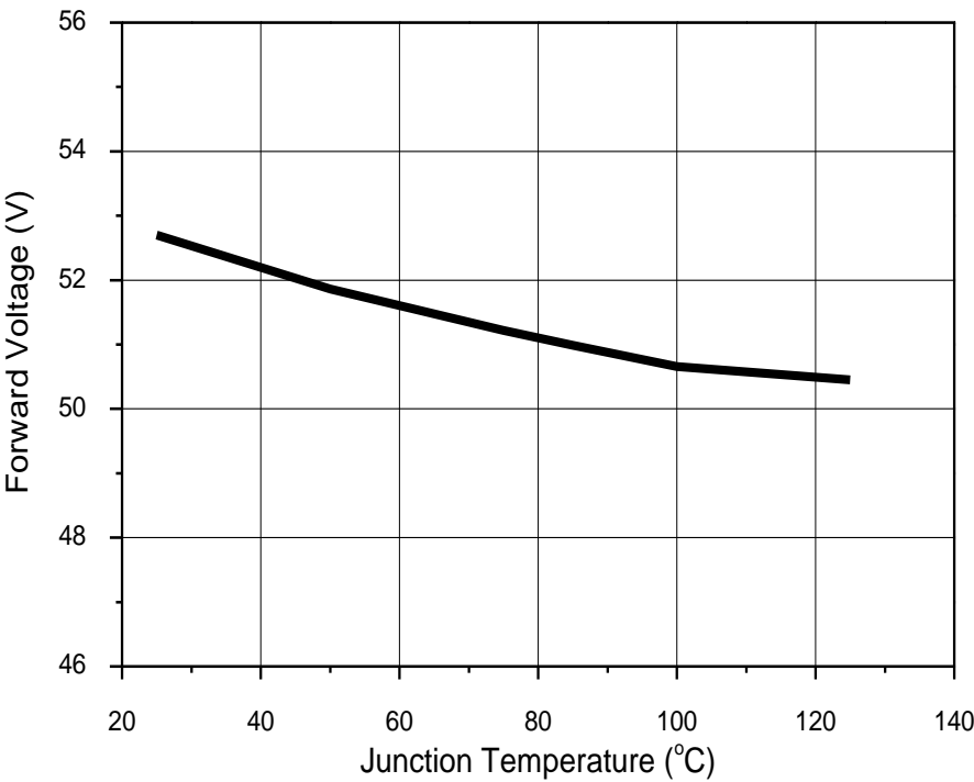
Fig 7. Forward Voltage vs. Junction Temperature, I_F=1.5A
